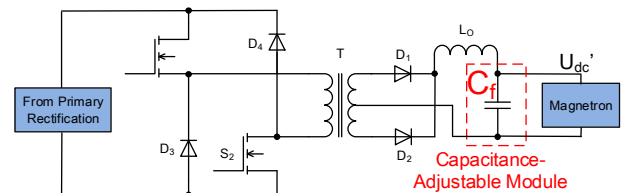
Fig. 2. The simplified schematic of a power supply.
