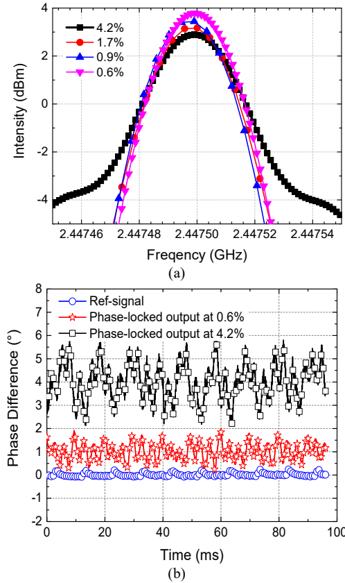
Fig. 6. Max-hold spectra (a) (Both RBW and VBW are 30 kHz.) and phase jitters (b) with respect to the various anode voltage ripples.
