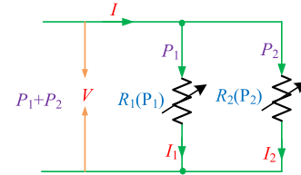
Fig. 1. Simplified mode of two shunt nonlinear resistances.
