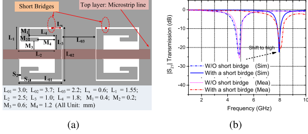
Fig. 3. BSF using DGS. (a) Physical dimension of the DGS with/without short birdies. (b) |S_{21}| of the BSF with/without metal short birdies.
