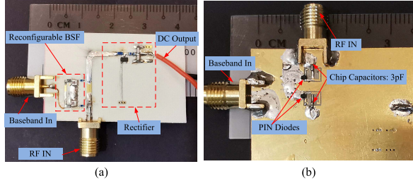
Fig. 6. Photograph of the fabricated IRT. (a) Top view. (b) Bottom view.
