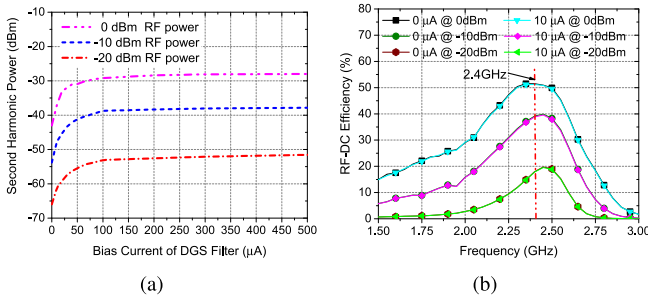
Fig. 8. (a) Measured second-harmonic level versus bias current. (b) Measured PCE versus RF frequency with/without 10- \mu A bias current.
