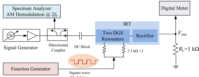
Fig. 7. Schematic of the experimental measurement setup.
