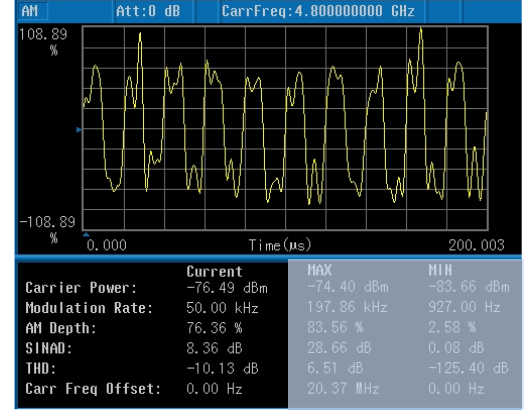
Fig. 9. Demodulated 50-kHz square-wave when the IRT has an RF input power of -20 dBm, a 20-dB coupler was used in experiments.
