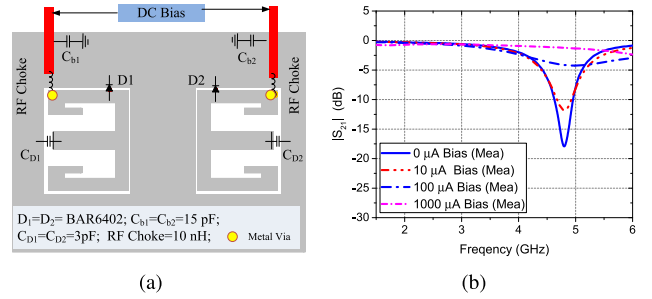
Fig. 4. (a) Bottom view of the reconfigurable BSF with p-i-n diodes and bias circuits. (b) Measured |S_{21}| with bias current of 0, 10, 100, and 1000 \mu\text{A} .
