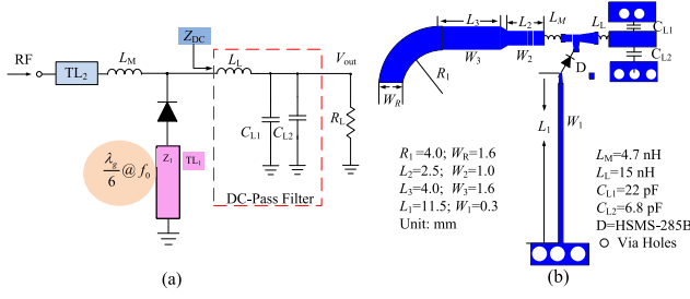
Fig. 5. Single-diode rectifier used in IRT. (a) Schematic. (b) Layout with design parameters.
