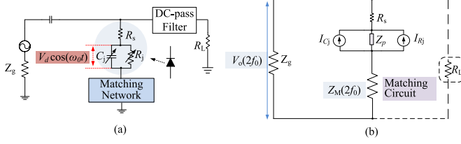
Fig. 2. (a) Block diagram of the single-diode rectifier used in IRT. (b) Diode servers as a second-harmonic source modeled by a Norton equivalent circuit.
