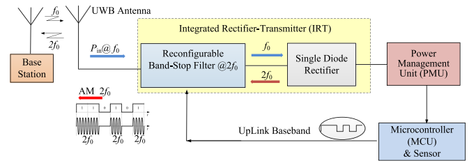
Fig. 1. System illustration of the proposed IRT, where the generated second harmonic ( 2f_0 ) is modulated and reradiates out through the antenna.
