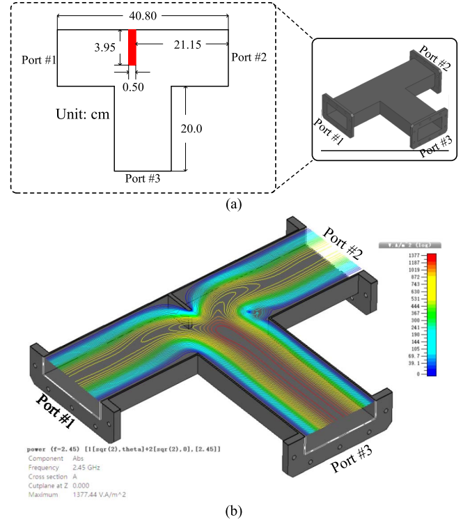
Fig. 2. (a) Physical dimensions of the designed asymmetric H-plane tee. (b) Power flow when the phase difference between the inputs is optimal in the CST environment.
