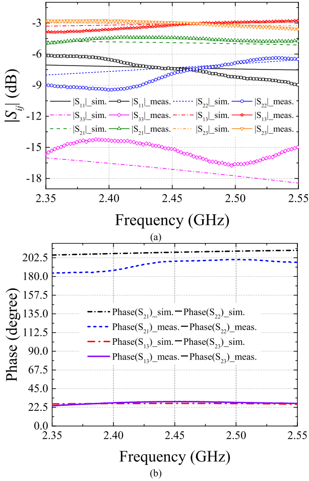
Fig. 3. Simulated and measured asymmetric H-plane tee. (a) Scattering parameters. (b) Phase differences.
