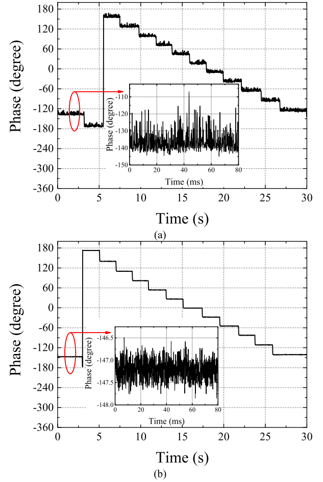
Fig. 10. Phase adjustment of the combining signal (a) when the EIL is turned on and (b) when both the EIL and CLPC are turned on.
