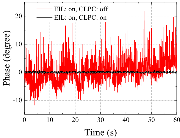
Fig. 11. Long-term comparison of phase jitters. The white dashed line is the x -axis of the chart.
