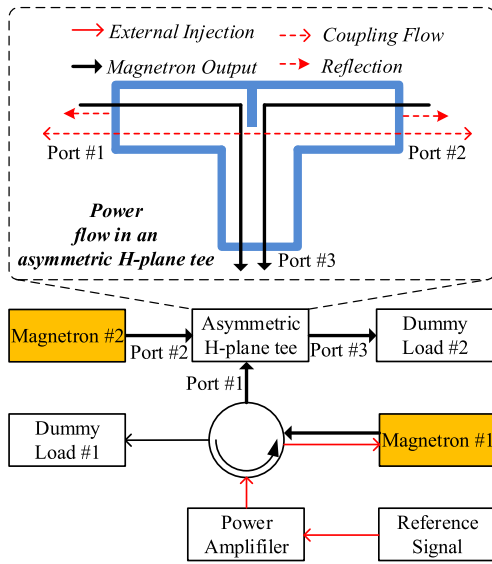
Fig. 1. Simplified schematic of the proposed dual-way magnetron combining system.
