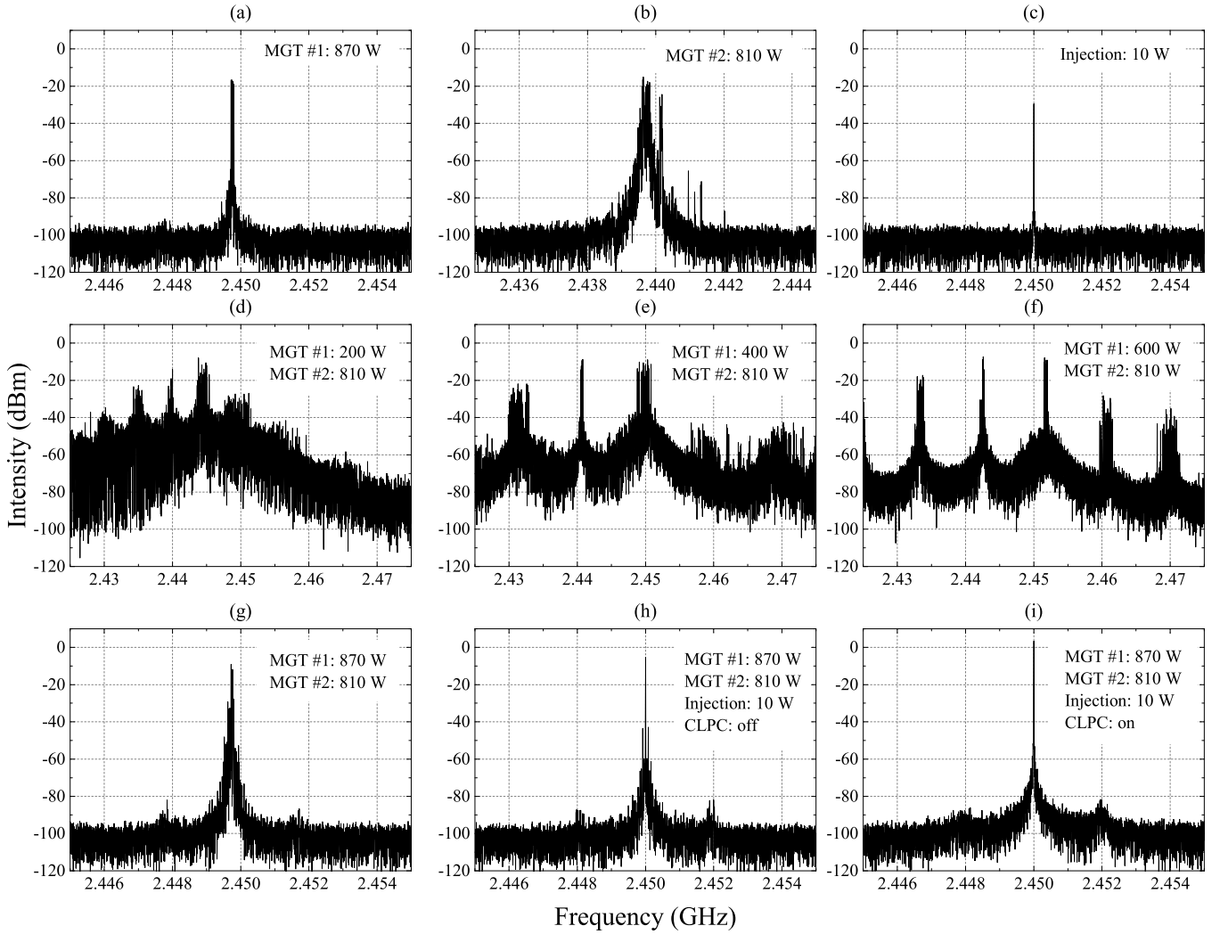
Fig. 8. Spectra of the proposed system in different conditions. The resolution bandwidth is 3 kHz, and the video bandwidth is 3 kHz.
