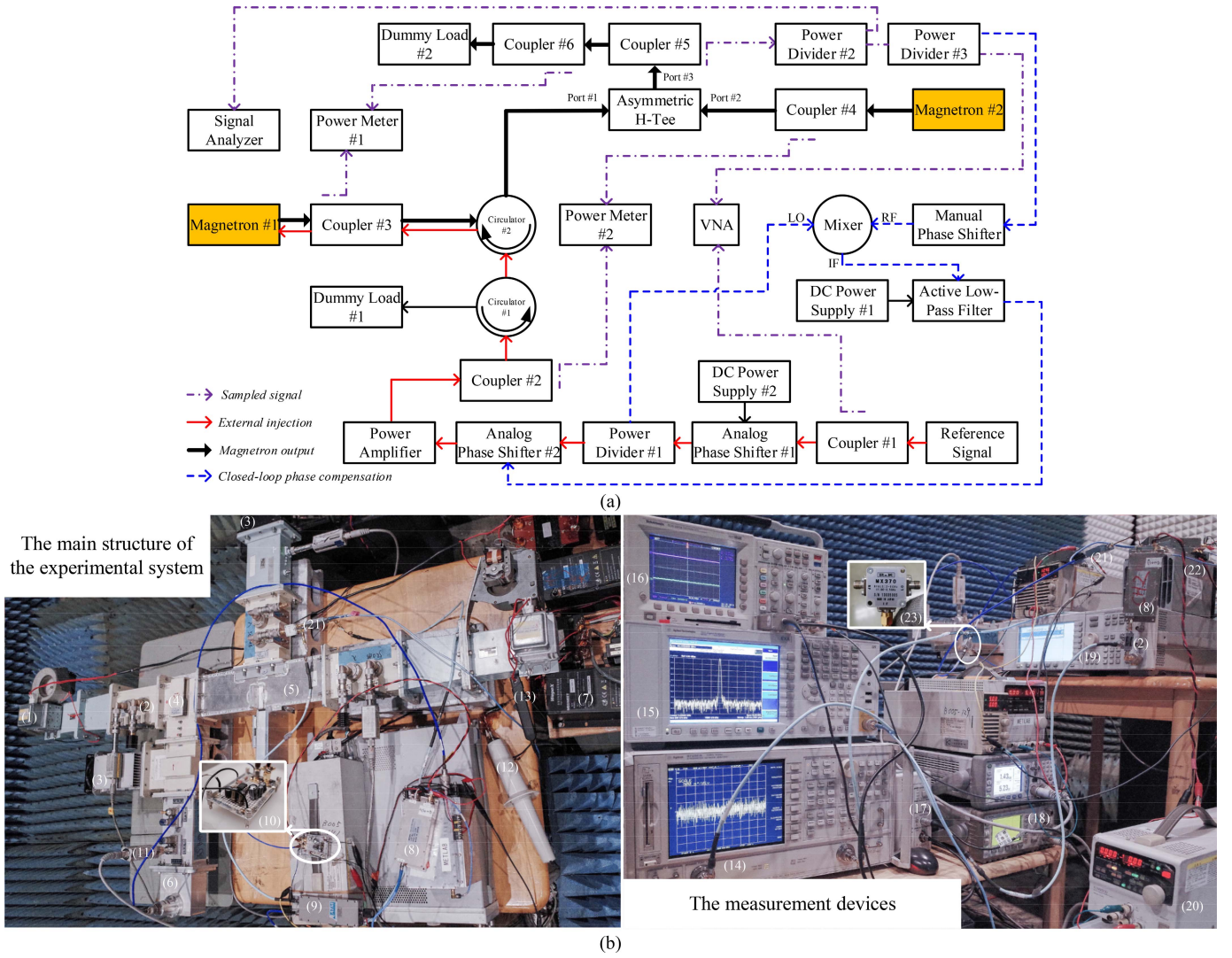
Fig. 7. (a) Block diagram of the experimental system and (b) photograph of the experiment setup. Components and devices: (1) magnetron, (2) coupler, (3) dummy load, (4) circulator, (5) asymmetric H-tee, (6) coaxial-to-waveguide converter, (7) magnetron's power supply, (8) analog phase shifter, (9) manual phase shifter, (10) active low-pass filter, (11) power sensor, (12) high-voltage probe, (13) current probe, (14) VNA, (15) signal analyzer, (16) oscilloscope, (17) current amplifier, (18) power meter, (19) signal generator, (20) dc power supply, (21) 1-to-2 power divider, (22) power amplifier, and (23) mixer.
