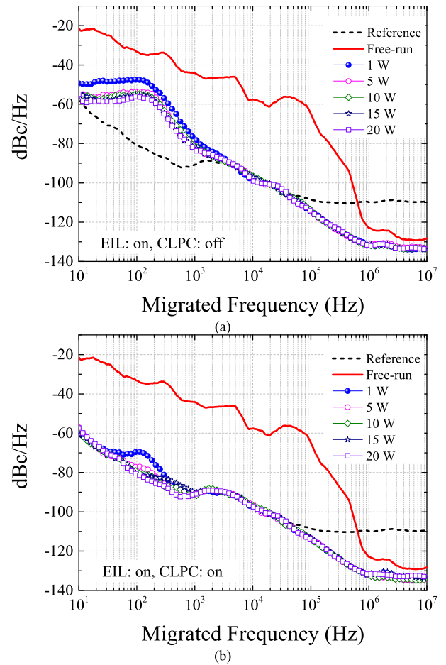
Fig. 12. Noise performances of combining the output with respect to the different external injection power. (a) EIL: on, CLPC: off; (b) EIL: on, CLPC: on.
