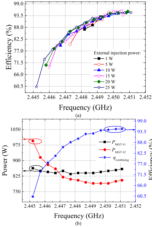
Fig. 9. (a) Measured power-combining efficiency with respect to the varied external injection frequency. (b) Power variations of two magnetrons and the combining efficiency with respect to the tuned frequency.
