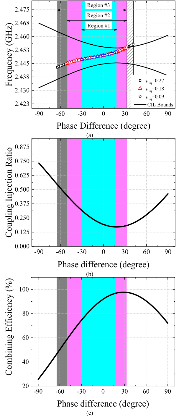
Fig. 4. Mapping relationships among the phase differences of the inputs, (a) frequency sweep scope, (b) coupling injection ratio, and (c) combining efficiency.
