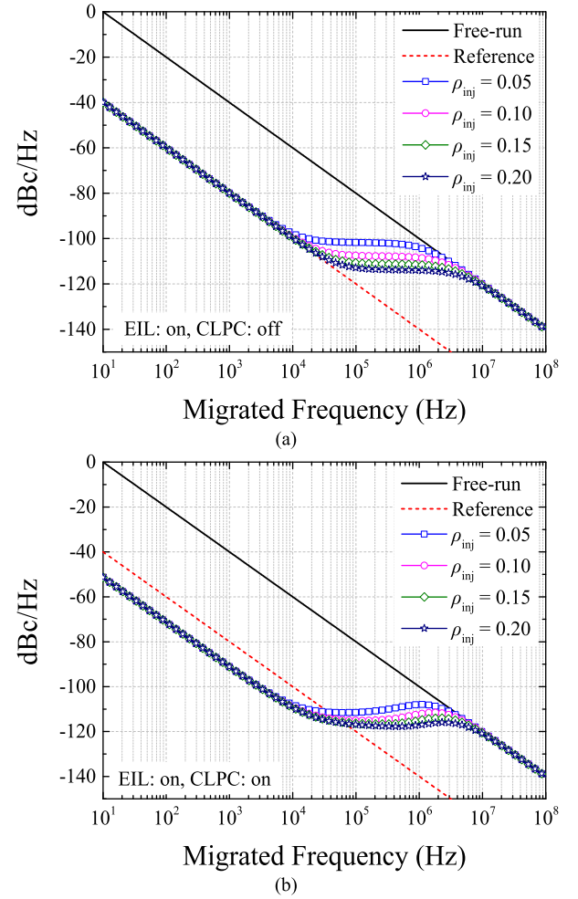
Fig. 6. (a) Characteristics of the relative output phase noise of the free-running oscillator, external injection source, and EIL magnetron. (b) Characteristics of the relative output phase noise of the free-running oscillator, external injection source, and EIL magnetron when the CLPC is activated.
