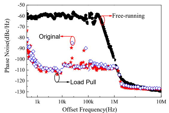
Fig. 4. The phase noise of the magnetron.
