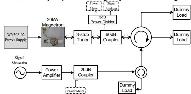
Fig. 1. Diagram of the injection-locked magnetron with the load-pull characterization system
