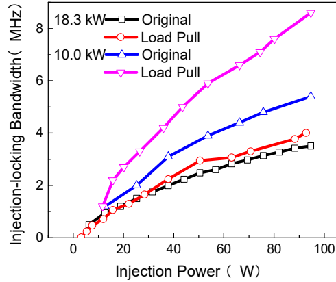
Fig. 3. The injection locked bandwidth with various injection ratios at different state.
