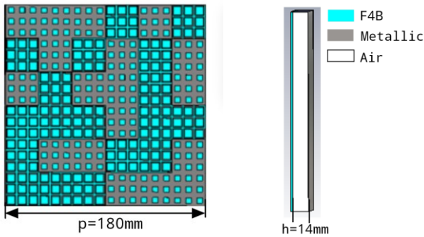
Figure 3. Random layout of 1-bit coding metasurface with dimension size of 180 mm \times 180 mm \times 16 mm (14 mm-thick air layer and 2 mm-thick F4B substrate)
