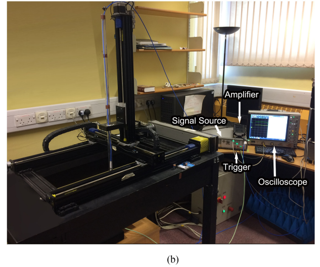
Fig. 2. Time-domain near-field scanning system. (a) Structural diagram. (b) In the University of Nottingham.
