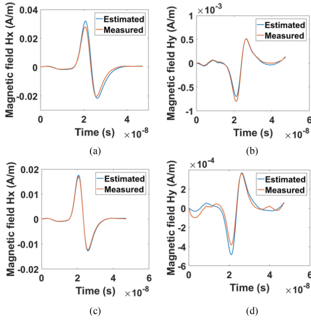
Fig. 8. Measured and estimated tangential magnetic fields of the selected observation point at two scanning heights. (a) H_x(t) above TL 5 mm. (b) H_y(t) above TL 5 mm. (c) H_x(t) above TL 10 mm. (d) H_y(t) above TL 10 mm.
