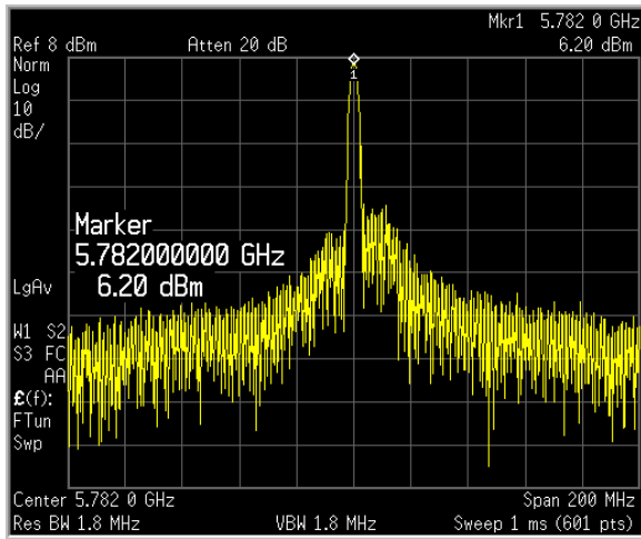
Fig. 16. Spectrum of the four-way magnetron power-combining signal.
