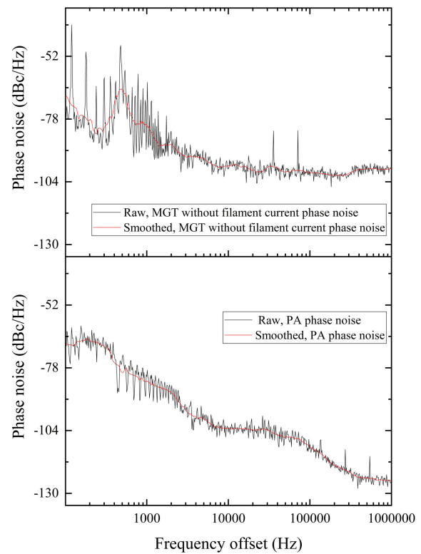
Fig. 11. Phase noise of the phase-locked magnetron.
