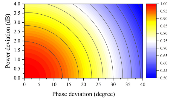
Fig. 7. Power-combining efficiency with power and phase deviations.
