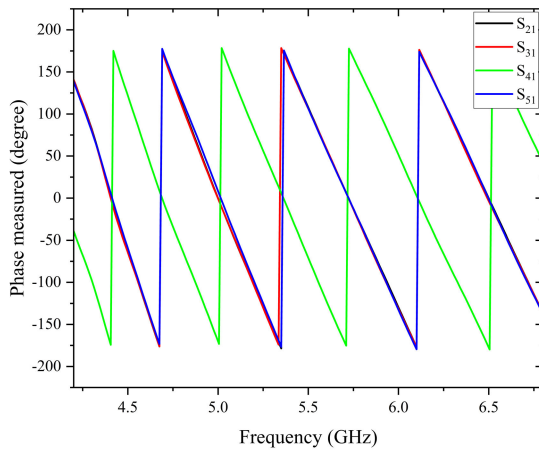
Fig. 5. Measured phase characteristics between port 1 and ports 2–5.
