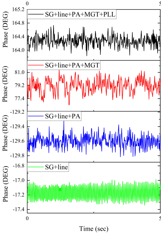
Fig. 12. Phase measurement of the phase-locked magnetron.
