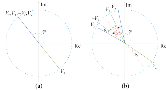
Fig. 6. Phase and amplitude of microwave at each input port. (a) Ideal power-combining state. (b) Practical power-combining state.
