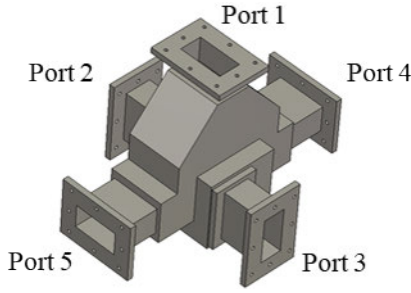
Fig. 1. Model of the four-way combiner.
