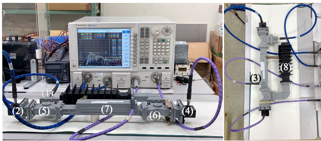
Fig. 14. Parts of the injection-locked magnetron subsystem. 1—port for the injected signal, 2—port connected to the magnetron, 3—port for connecting the power meter, 4—port connected to the combiner, 5 and 6—circulators, 7—directional coupler, and 8—dummy load.
