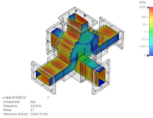
Fig. 2. Electronic field of the four-way combiner.
