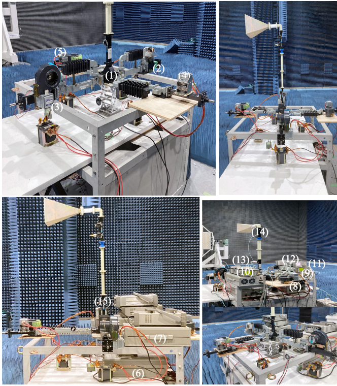
Fig. 15. Photographs of the combining experiment. 1—five-port combiner, 2–5—parts of injection-locked magnetron subsystem, 6–9—power amplifiers, 10–12—power meters, 13—phase shifter, 14—50-dB directional coupler b, and 15—50-dB directional coupler a.
