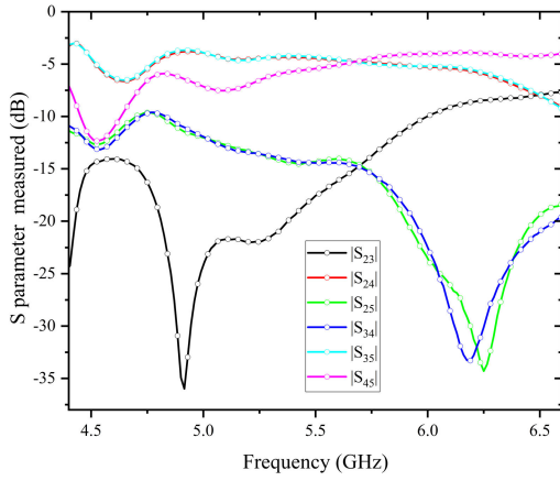
Fig. 4. Measured S -parameter characteristics among ports 2–5.
