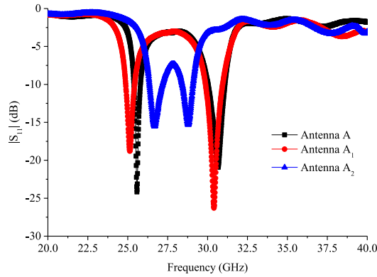
Fig. 9. Measured input reflection coefficients of antennas A, A 1 , and A 2 .
