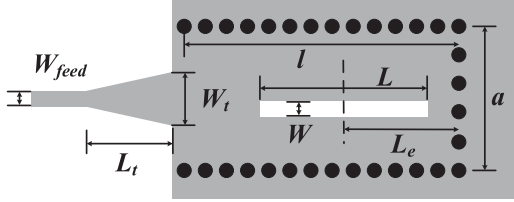
Fig. 2. Proposed dual-frequency single-slot antenna A.
