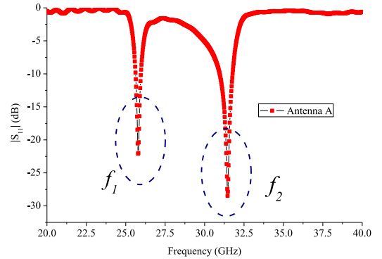
Fig. 4. Simulated comparison of input reflection coefficients ( |S_{11}| ) of antenna A.
