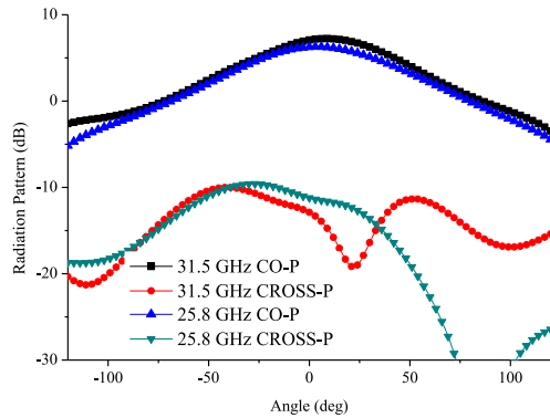
Fig. 6. Radiation pattern at 25.8 and 31.5 GHz of antenna A.
