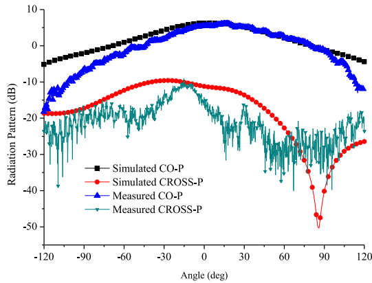
Fig. 10. Measured radiation pattern of antenna A of 25.3 GHz.
