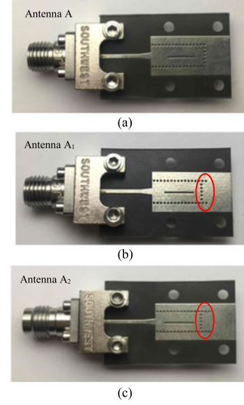
Fig. 7. Fabricated antennas: (a) the proposed dual-band antenna A, (b) and (c) the dual-band antennas A 1 and A 2 with shifted SIW length for frequency adjustment.
