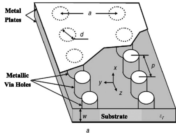
Fig. 1. Basic structure and parameters of the SIW.
