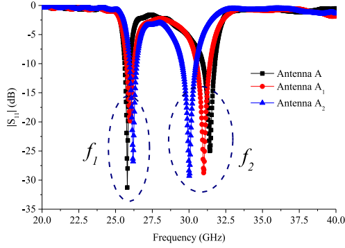
Fig. 5. Input reflection coefficients of antennas A, A 1 , and A 2 , which shows the possibility for frequency adjustment.
