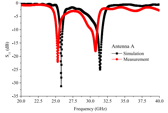
Fig. 8. Measured and simulated input reflection coefficients of antenna A.
