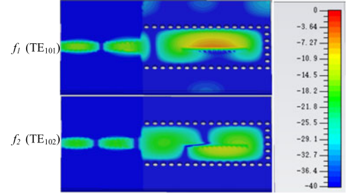
Fig. 3. Electric field distribution of the proposed antenna A of two modes on two resonance frequencies.
