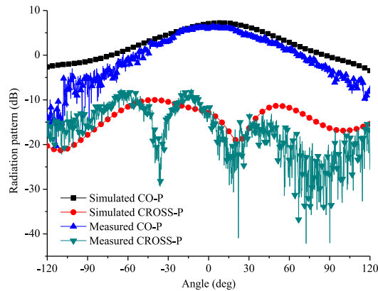
Fig. 11. Measured radiation pattern of antenna A of 30.76 GHz.
