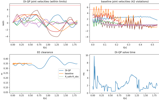
Fig. 5. 7-DOF FR3 dynamic obstacle. Top-left: DI-QP joint velocities, all within the limit. Top-right: resolved-rate+APF baseline, which exceeds the velocity limit. Bottom-left: end-effector clearance. Bottom-right: DI-QP per-cycle solve time.
