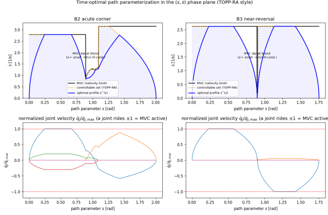
Fig. 2. Time-optimal path parameterization in the (s, \dot{s}) phase plane (TOPP-RA style). The optimal profile dips at the tight blend and—on the near-reversal—plunges to \dot{s} \approx 0 , exactly where the s \rightarrow t map becomes singular.
