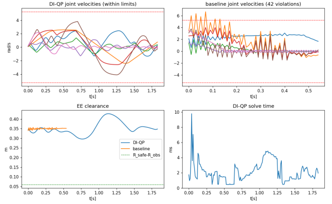
Fig. 3. 7-DOF FR3 dynamic obstacle. Top-left: DI-QP joint velocities, all within the limit. Top-right: resolved-rate+APF baseline, which exceeds the velocity limit. Bottom-left: end-effector clearance. Bottom-right: DI-QP per-cycle solve time.
