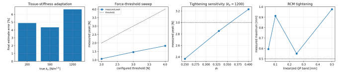
Fig. 5. Multi-condition verification: tissue-stiffness estimation, configured force-threshold sweep, empirical \rho_F sensitivity, and RCM-band tightening.
