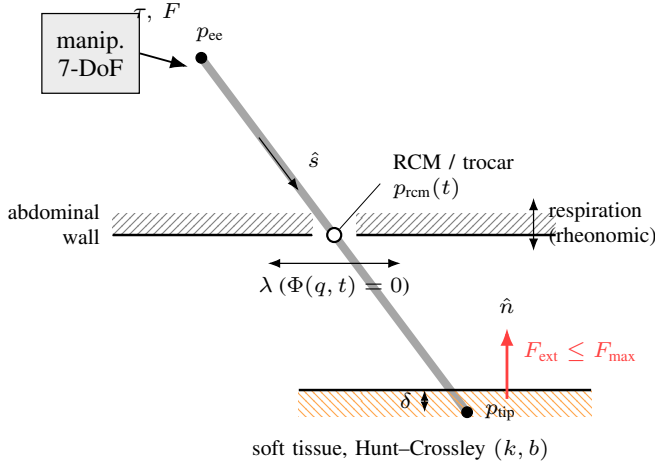
Fig. 1. RCM-constrained laparoscopic plant, mapping the variables of this section onto the physical parts: a 7-DoF manipulator applies joint torque \tau and tip force F (1) through a rigid instrument with flange p_{ee} , tip p_{tip} , and shaft direction \hat{s} . The instrument pivots about the trocar incision—the remote center of motion p_{rcm}(t) , which may vary in the general model but is fixed in the experiments—where the lateral deviation \Phi(q, t) (2) must be held at zero against the lateral trocar force \lambda . The tip presses on soft tissue modeled by Hunt–Crossley contact (stiffness k , damping b , penetration \delta ) (4), producing the contact force F_{ext} regulated relative to the configured force limit F_{max} along the contact normal \hat{n} . The implemented respiratory disturbance moves the planar tissue surface along the shaft direction.
