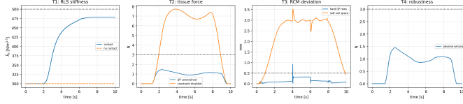
Fig. 4. Verification tests T1–T4: adaptive RLS and no-contact gating; force limitation under a deep reference; decision-coupled versus soft RCM regulation; and adverse sensing with stick-slip friction.
