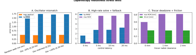
Fig. 6. Robustness stress tests: oscillator/frequency mismatch (A), configured actuator delay with fallback (B), and trocar deadzone with stick–slip friction (C).
