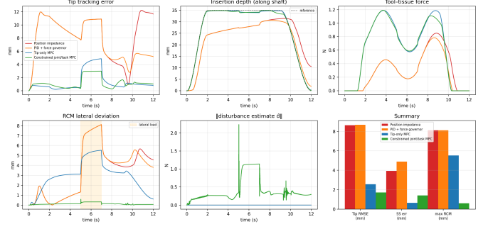
Fig. 2. Palpation benchmark through a compliant, respiring trocar: tip tracking error, insertion depth, tool-tissue force, RCM lateral deviation, diagnostic residual estimate, and summary metrics for the four controllers of Table I.
