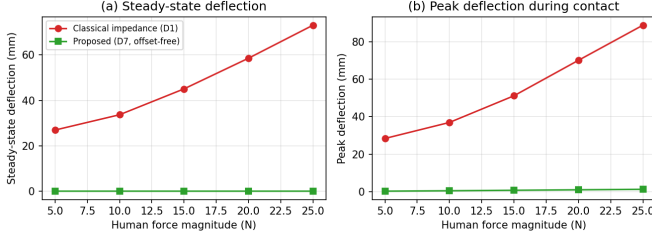
Fig. 4. Human-force magnitude sweep: steady-state (a) and peak (b) tip deflection versus a sustained push, for classical impedance (D1, red) and the proposed offset-free controller (D7, green). The proposed steady-state deflection is invariant to force magnitude.
