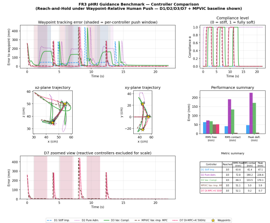
Fig. 2. Benchmark II — reach-and-hold under directionally varied push. For visibility the plot shows D1/D2/D3/D7 (corresponding to G1/G2/G3/G7) plus the predictive variable-impedance MPVIC baseline; Table V reports the full ablation. The final D7 controller reaches every waypoint with sub-millimeter contact-window deflection.
