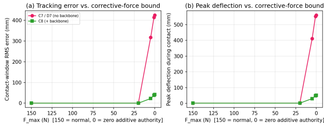
Fig. 5. Correction-authority robustness ablation: contact-window RMS (a) and peak deflection (b) versus the QP’s corrective-force bound F_{\max} , with (C8, green) and without (C7, red) the impedance backbone. C8 degrades gracefully as F_{\max} \rightarrow 0 while C7 collapses toward bare feedforward.
