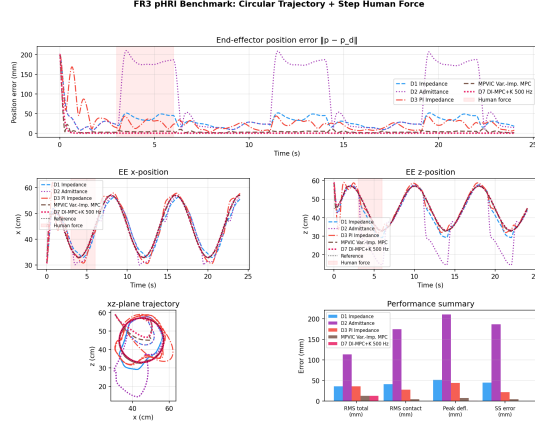
Fig. 1. Benchmark I — Circular trajectory under 15N step pHRI. For visibility the plot shows D1/D2/D3/D7 (corresponding to C1/C2/C3/C7) plus the predictive variable-impedance MPVIC baseline; Table III reports the full ablation. The final D7 controller achieves near-zero steady-state error and sub-millimeter peak deflection, while MPVIC—though predictive—retains a visible steady-state offset.
