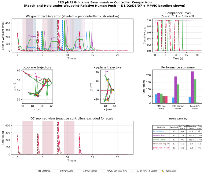
Fig. 2. Benchmark II — reach-and-hold under directionally varied push. For visibility the plot shows D1/D2/D3/D7 (corresponding to G1/G2/G3/G7) plus the predictive variable-impedance MPVIC baseline; Table V reports the full ablation. The final D7 controller reaches every waypoint with sub-millimeter contact-window deflection.
