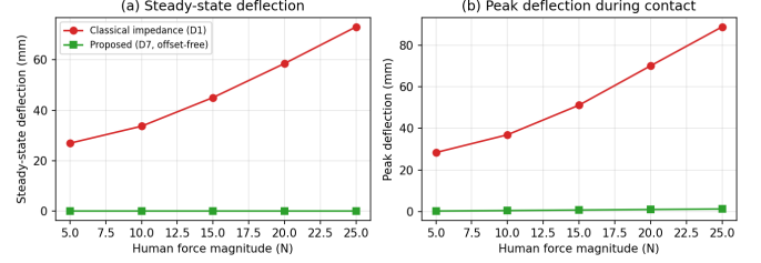
Fig. S2. Human-force magnitude sweep: steady-state (a) and peak (b) tip deflection versus a sustained push, for classical impedance (D1, red) and the proposed offset-free controller (D7, green). The proposed steady-state deflection is invariant to force magnitude (0.023 mm), while classical impedance grows linearly.
