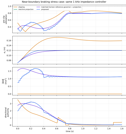
Fig. 3. Near-boundary braking stress case.
