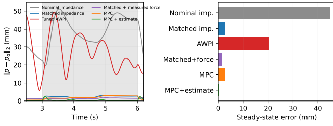
Fig. 2. Evaluation-cycle fair comparison. Stiffness/damping calibration closes the nominal impedance/C4 steady-state gap. The controlled C4–C5 pair isolates the disturbance augmentation; ideal measured-force feedforward also reduces the load-axis bias but retains the matched impedance’s saturation and power cost.
