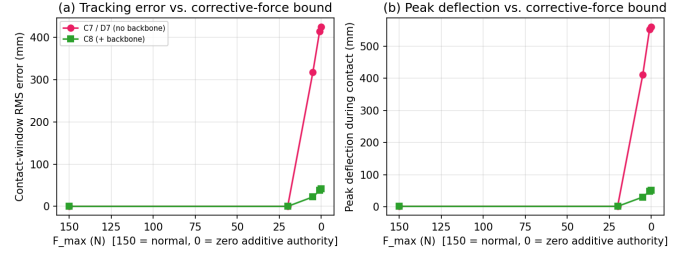
Fig. 3. Correction-authority robustness ablation: contact-window RMS (a) and peak deflection (b) versus the QP’s corrective-force bound F_{\text{max}} , for the proposed controller with (C8, green) and without (C7, red) the impedance backbone. C8 degrades gracefully as F_{\text{max}} \rightarrow 0 while C7 collapses toward bare feedforward.
