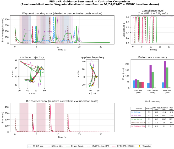
Fig. S1. Benchmark II — reach-and-hold under directionally varied push. For visibility the plot shows D1/D2/D3/D7 (corresponding to G1/G2/G3/G7) plus the predictive variable-impedance MPVIC baseline; Table S3 reports the full ablation. The final D7 controller reaches every waypoint with sub-millimeter contact-window deflection.
