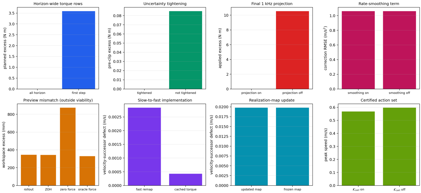
Fig. 6 isolates the four design choices central to the paper. Full-horizon enforcement keeps the horizon-ramp QP feasible and removes the 3.587 N m planned violation left by first-step-only enforcement. Removing uncertainty tightening creates 0.0848 N m of pre-clip excess; removing the final projection creates 10.538 N m of applied excess under sudden disturbance. In the dedicated velocity-bound case, enforcing \mathcal{K}_v limits peak speed to 0.5678 m/s, versus 0.5968 m/s without it. Appendix A gives the complete 17-run ablation ledger, secondary results, and wall-clock computation figures.
