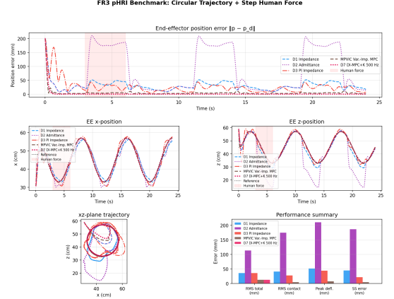
Fig. 1. Benchmark I — Circular trajectory under 15 N step pHRI. For visibility the plot shows D1/D2/D3/D7 (corresponding to C1/C2/C3/C7) plus the predictive variable-impedance MPVIC baseline; Table III reports the full ablation. The final D7 controller achieves near-zero steady-state error and sub-millimeter peak deflection, while MPVIC—though predictive—retains a visible steady-state offset.
