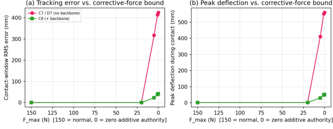
Fig. 3. Correction-authority robustness ablation: contact-window RMS (a) and peak deflection (b) versus the QP’s corrective-force bound F_{\max} , for the proposed controller with (C8, green) and without (C7, red) the impedance backbone. C8 degrades gracefully as F_{\max} \rightarrow 0 while C7 collapses toward bare feedforward.
