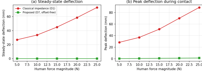
Fig. 2. Human-force magnitude sweep: steady-state (a) and peak (b) tip deflection versus a sustained push, for classical impedance (D1, red) and the proposed offset-free controller (D7, green). The proposed steady-state deflection is invariant to force magnitude (0.021 mm), while classical impedance grows linearly.
