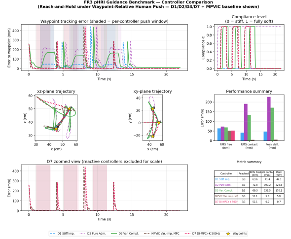
Fig. 1. Benchmark II — reach-and-hold under directionally varied push. For visibility the plot shows D1/D2/D3/D7 (corresponding to G1/G2/G3/G7) plus the predictive variable-impedance MPVIC baseline; Table III reports the full ablation. The final D7 controller reaches every waypoint with sub-millimeter contact-window deflection.
