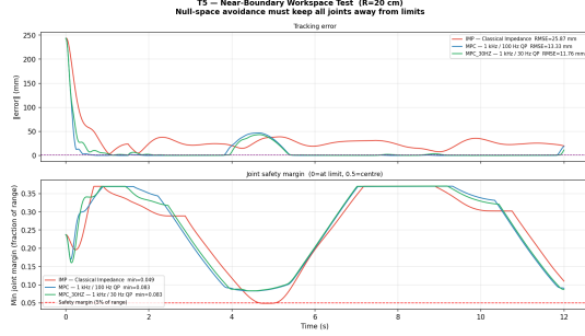
Fig. 3. Boundary test ( R = 20 cm). Classical impedance violates the 5% joint margin; the dual-barrier MPC maintains a fractional joint margin \geq 0.083 throughout. Elevated RMSE (13.3 mm) reflects the workspace projection intentionally offsetting p_d by up to 6 cm to maintain joint-limit clearance.
