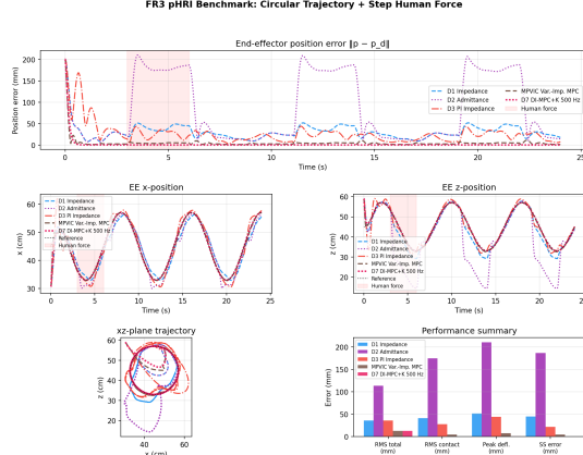
Fig. 1. Benchmark I — Circular trajectory under 15 N step pHRI. For visibility the plot shows D1/D2/D3/D7 (corresponding to C1/C2/C3/C7) plus the predictive variable-impedance MPVIC baseline; Table III reports the full ablation. The final D7 controller achieves near-zero steady-state error and sub-millimeter peak deflection, while MPVIC—though predictive—retains a visible steady-state offset.
