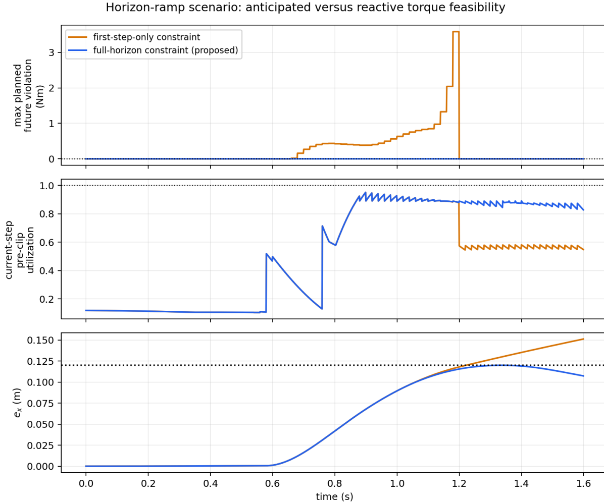
Fig. 1 isolates why anticipation is a different constraint from reactive limiting, not a refinement of it:
