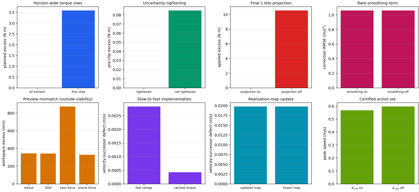
Fig. 7 isolates the four design choices central to the paper. Full-horizon enforcement keeps the horizon-ramp QP feasible and removes the 3.587 N m planned violation left by first-step-only enforcement. Removing uncertainty tightening creates 0.0848 N m of pre-clip excess; removing the final projection creates 10.538 N m of applied excess under sudden disturbance. In the dedicated velocity-bound case, enforcing K_v limits peak speed to 0.5678 m/s, versus 0.5968 m/s without it. Appendix A gives the complete 17-run ablation ledger and secondary results.
