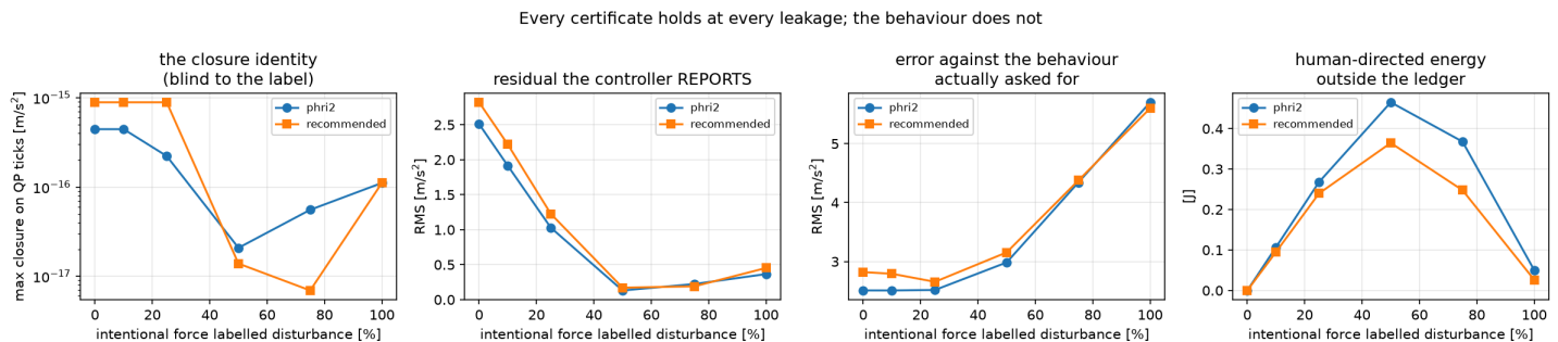
Figure 12 — the pillar. Panels 2 and 3 are the result: the residual the controller reports falls while the error against the behaviour actually asked for rises. The two poses almost coincide, which is worth noting on its own after §11.1’s table — this is the one finding here that is not a property of one FR3 configuration.
