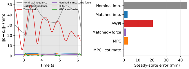
Fig. 2. Evaluation-cycle fair comparison. Stiffness/damping calibration closes the nominal impedance/C4 steady-state gap. The controlled C4–C5 pair isolates the disturbance augmentation; ideal measured-force feedforward also reduces the load-axis bias but retains the matched impedance’s saturation and power cost.
