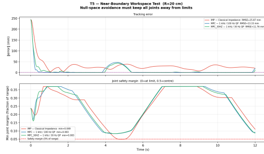
Fig. 3. Boundary-circle trajectories. The workspace correction trades tracking accuracy for clearance: the nominal impedance crosses the selected 5% fractional margin (minimum 0.049), whereas C5 maintains 0.083 in this test. The plotted result exercises the soft mechanisms in (16)–(17), not the optional CBF.
