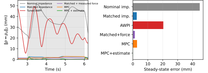
Fig. 2. Held-out fair comparison. Response matching closes the nominal impedance/C4 steady-state gap. The controlled C4–C5 pair isolates the disturbance augmentation; ideal measured-force feedforward also reduces the load-axis bias but retains the matched impedance’s saturation and power cost.
