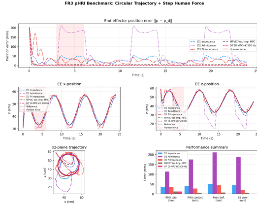
Fig. 1. Representative trajectories from the broad screen. The compliant admittance response is intentional; its large displacement is not a failure for a guidance task, but it is unsuitable for the reference-holding objective studied here. The response-matched study below removes the largest stiffness confound between impedance and MPC.
