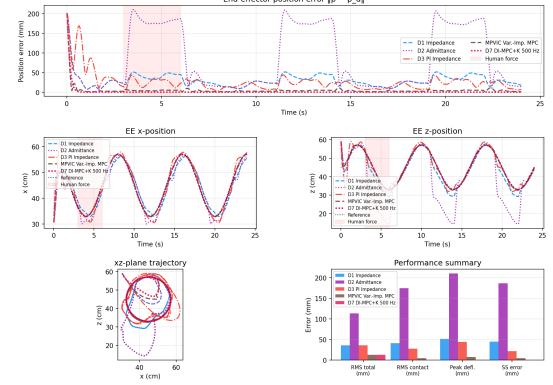
Fig. 1. Benchmark I — Circular trajectory under 15 N step pHRI. For visibility the plot shows D1/D2/D3/D7 (corresponding to C1/C2/C3/C7) plus the predictive variable-impedance MPVIC baseline; Table III reports the full ablation. The final D7 controller achieves near-zero steady-state error and sub-millimeter peak deflection, while MPVIC—though predictive—retains a visible steady-state offset.
