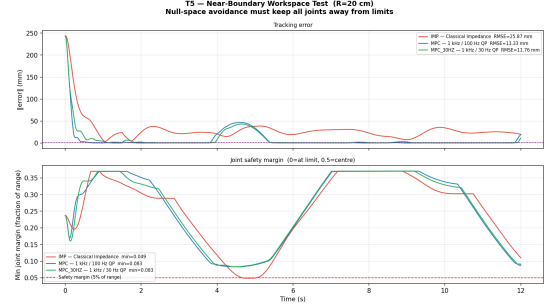
Fig. 3. Boundary test ( R = 20 \text{ cm} ). Classical impedance violates the 5% joint margin; the dual-barrier MPC maintains a fractional joint margin \geq 0.083 throughout. Elevated RMSE (13.3 mm) reflects the workspace projection intentionally offsetting p_d by up to 6 cm to maintain joint-limit clearance.
