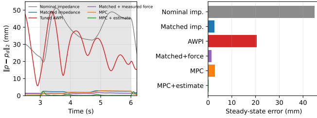
Fig. 2. Held-out three-cycle fair comparison. Calibration largely closes the nominal-impedance/C4 gap, whereas the C4–C5 pair isolates the effect of force-domain disturbance augmentation. Direct measured-force feedforward also removes most load-axis bias, while the matched impedance realizations briefly saturate and reach substantially higher peak positive joint power.
