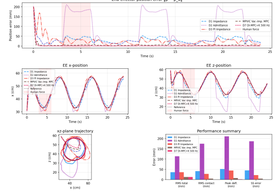
Fig. 1. Benchmark I — Circular trajectory under 15 N step pHRI. For visibility the plot shows D1/D2/D3/D7 (corresponding to C1/C2/C3/C7) plus the predictive variable-impedance MPVIC baseline; Table IV reports the full ablation. The final D7 controller achieves near-zero steady-state error and sub-millimeter peak deflection, while MPVIC—though predictive—retains a visible steady-state offset.
