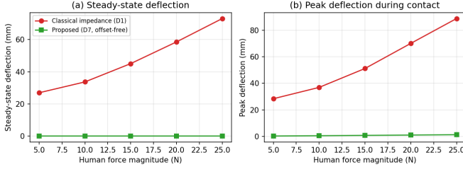
Fig. S2. Human-force magnitude sweep: steady-state (a) and peak (b) tip deflection versus a sustained push, for classical impedance (D1, red) and the proposed offset-free controller (D7, green). The proposed steady-state deflection is invariant to force magnitude (0.021 mm), while classical impedance grows linearly.
