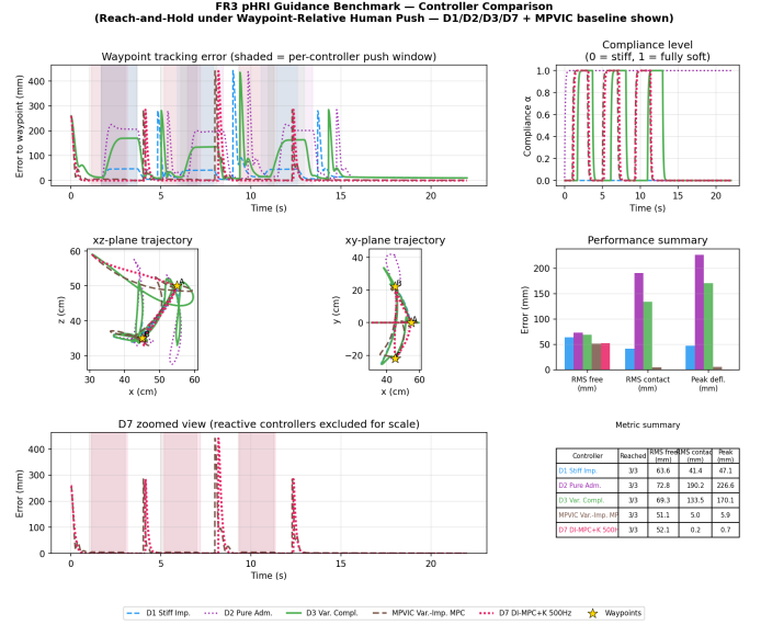
Fig. S1. Benchmark II — reach-and-hold under directionally varied push. For visibility the plot shows D1/D2/D3/D7 (corresponding to G1/G2/G3/G7) plus the predictive variable-impedance MPVIC baseline; Table S3 reports the full ablation. The final D7 controller reaches every waypoint with sub-millimeter contact-window deflection.
