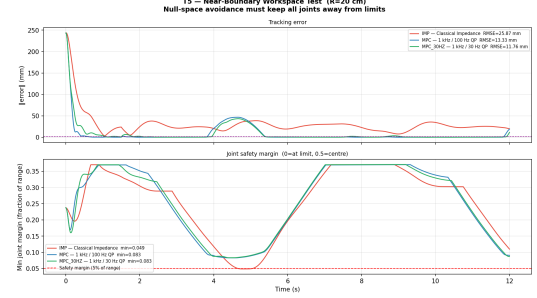
Fig. 3. Boundary-circle trajectories. The workspace correction trades tracking accuracy for clearance: the nominal impedance crosses the selected 5% fractional margin (minimum 0.049), whereas C5 maintains 0.083 in this test. The plotted result exercises the soft mechanisms in (16)–(17), not the optional CBF.
