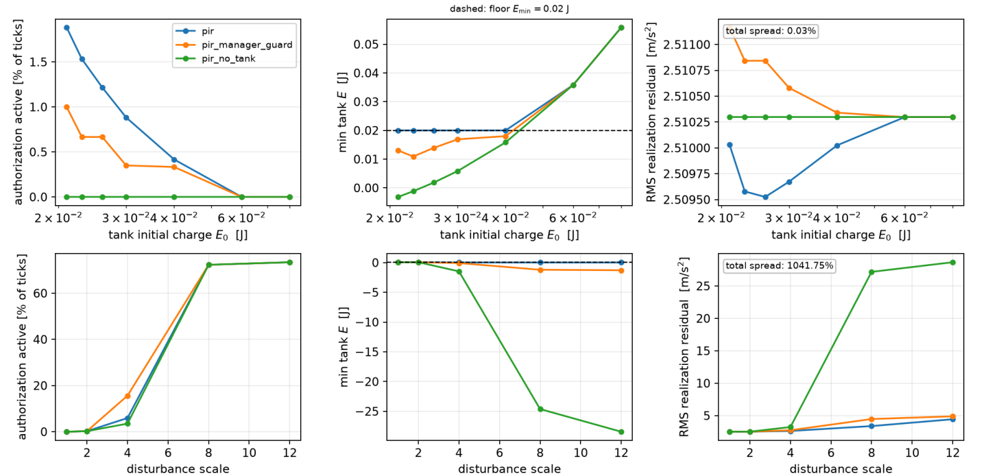
PIR: authorization vs tracking with both tightenings active ( K_0 = 380.0 N/m, D_0 = 29.07 N·s/m, envelope derated_joint4)
