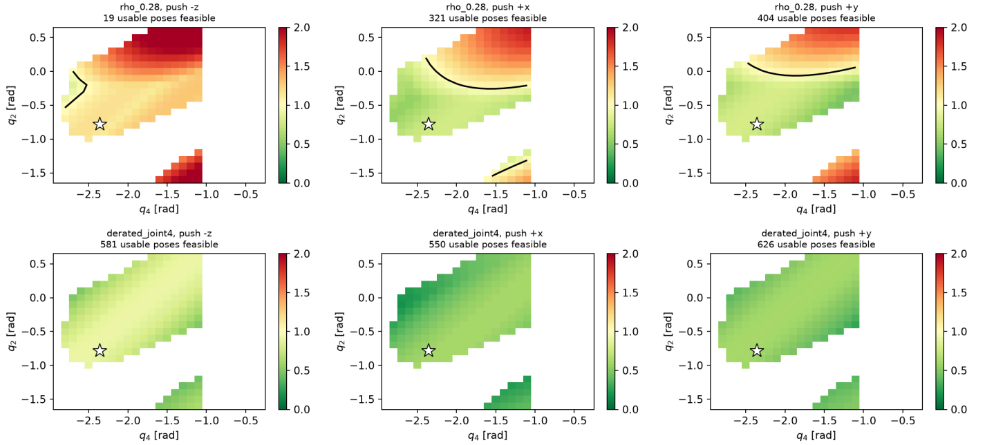
Figure 6 — the pose screen. Anchor proxy over (q_2, q_4) at q_6 = 1.571 , per envelope and push direction. The star is phri2's own pose. Blank cells are rejected by the controllability guard — poses that resist the push through kinematic structure rather than control, which the unguarded screen preferred. Green is not yet a verdict: §9.1's second trap means these still have to survive an along-trajectory replay.
