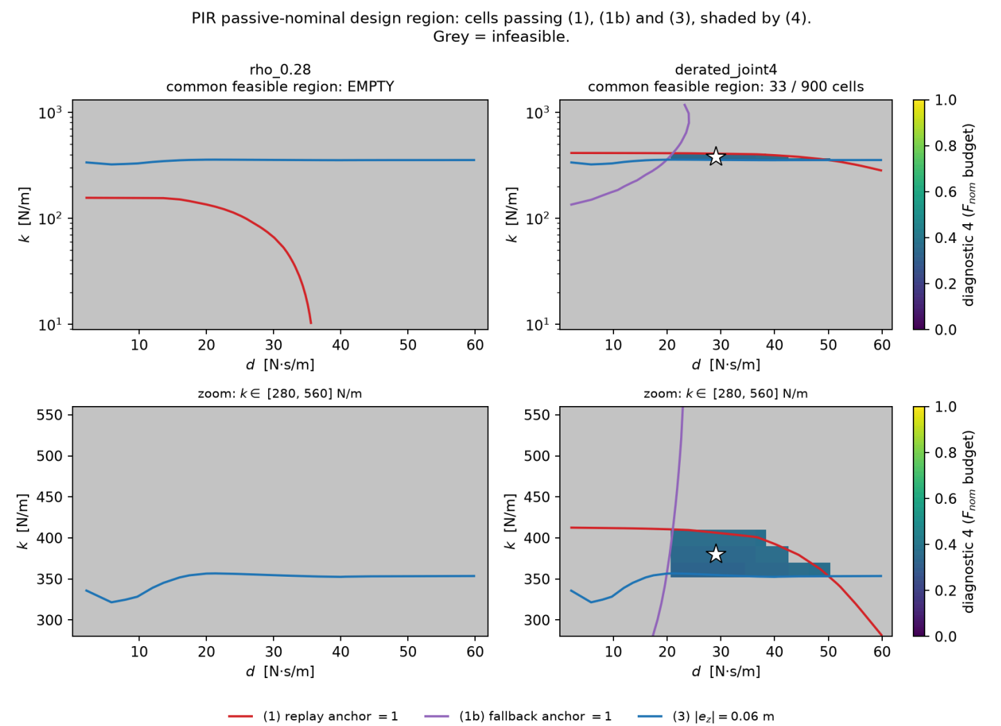
Figure 1 — the design region. Grey is infeasible. Left: the \rho = 0.28 envelope, empty everywhere. Right: phri2 ’s derated-joint-4 envelope, 33 of 900 cells, with the recommended operating point starred. The zoom row is not decoration — the region is \sim 40
