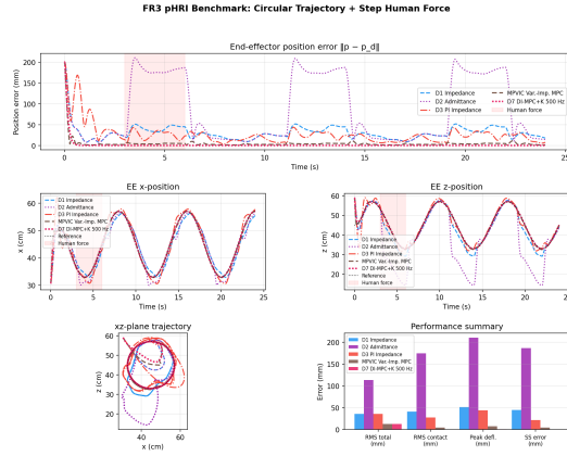
Fig. 1. Representative trajectories from the broad screen. The compliant admittance response is intentional; its large displacement is not a failure for a guidance task, but it is unsuitable for the reference-holding objective studied here. The response-matched study below removes the largest stiffness confound between impedance and MPC.
