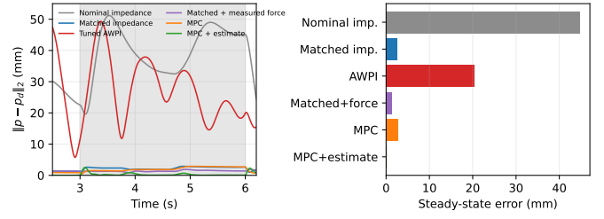
Fig. 2. Held-out fair comparison. Response matching closes the nominal impedance/C4 steady-state gap. The controlled C4–C5 pair isolates the disturbance augmentation; ideal measured-force feedforward also reduces the load-axis bias but retains the matched impedance’s saturation and power cost.
