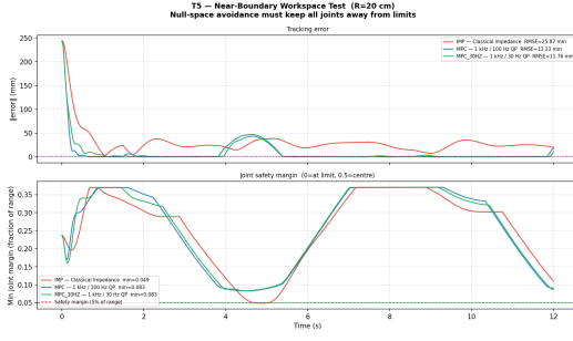
Fig. 3. Boundary-circle trajectories. The workspace correction trades tracking accuracy for clearance: the nominal impedance crosses the selected 5% fractional margin (minimum 0.049), whereas C5 maintains 0.083 in this test. The plotted result exercises the soft mechanisms in (16)–(17), not the optional CBF.
