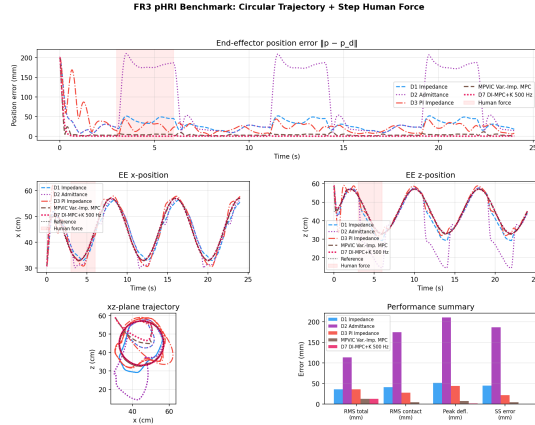
Fig. 1. Benchmark I — Circular trajectory under 15N step pHRI. For visibility the plot shows D1/D2/D3/D7 (corresponding to C1/C2/C3/C7) plus the predictive variable-impedance MPVIC baseline; Table IV reports the full ablation. The final D7 controller achieves near-zero steady-state error and sub-millimeter peak deflection, while MPVIC—though predictive—retains a visible steady-state offset.
