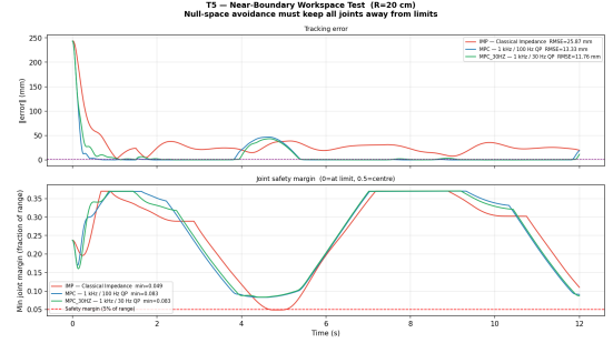
Fig. 3. Boundary test ( R = 20 cm). Classical impedance violates the 5% joint margin; the dual-barrier MPC maintains a fractional joint margin \geq 0.083 throughout. Elevated RMSE (13.3 mm) reflects the workspace projection intentionally offsetting p_d by up to 6 cm to maintain joint-limit clearance.
