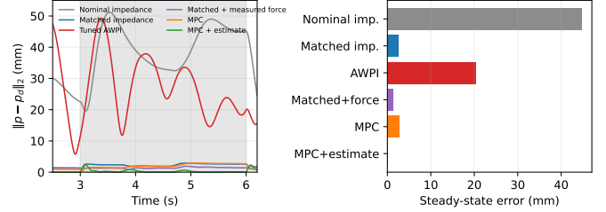
Fig. 2. Evaluation-cycle fair comparison. Stiffness/damping calibration closes the nominal impedance/C4 steady-state gap. The controlled C4–C5 pair isolates the disturbance augmentation; ideal measured-force feedforward also reduces the load-axis bias but retains the matched impedance's saturation and power cost.
