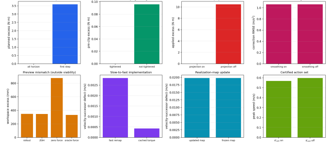
Fig. 6. Paired ablations of the predictive and fast-path implementation choices.
