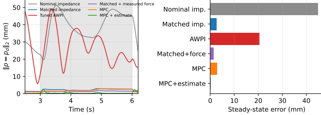
Fig. 1. Evaluation-cycle fair comparison. Stiffness/damping calibration closes the nominal impedance/C4 steady-state gap. The controlled C4–C5 pair isolates the disturbance augmentation; ideal measured-force feedforward also reduces the load-axis bias but retains the matched impedance’s saturation and power cost.
