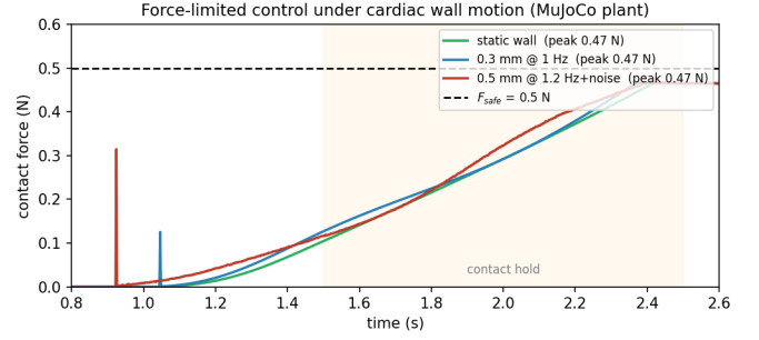
Fig. 3. Measured tissue force for the force-limited impedance-plus-integral controller under the three wall conditions of Table III. All tested peaks remain near 0.47 N; the result is specific to the modeled catheter tip motion, and approach profile.
