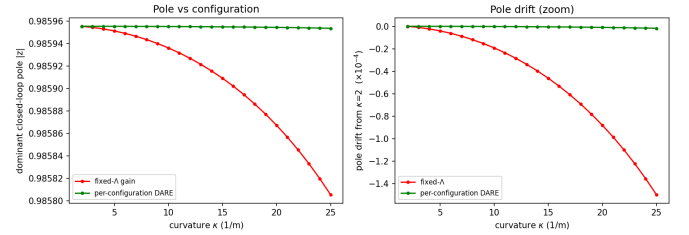
Fig. 4. Reduced-model dominant-pole magnitude and drift over curvature. Per-configuration DARE redesign (green) gives a 1.78 \times 10^{-6} spread for the stated weights, versus 1.50 \times 10^{-4} for the fixed nominal gain (red).
