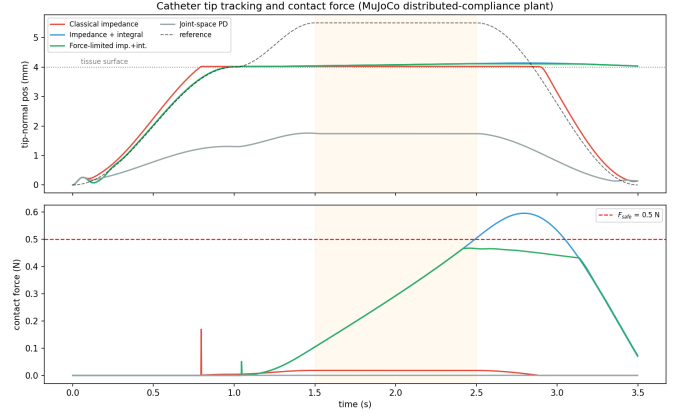
Fig. 2. Tip tracking (top) and measured Kelvin–Voigt tissue force (bottom) for the four controllers of Table I. The force-limited impedance-plus-integral controller (green) gives a 0.467 N measured peak under the configured 0.5 N threshold; removing the corrective-force limit (blue) raises the peak to 0.595 N. Classical impedance reaches 0.169 N with larger approach error, and joint-space PD does not reach the tissue in this task.
