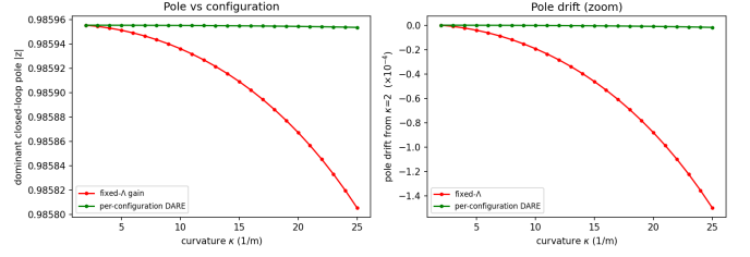
Fig. 4. Reduced-model dominant-pole magnitude and drift over curvature. Per-configuration DARE redesign (green) gives a 1.78 \times 10^{-6} spread for the stated weights, versus 1.50 \times 10^{-4} for the fixed nominal gain (red).
