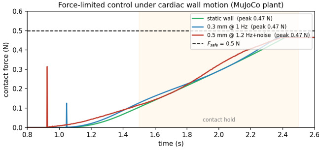
Fig. 3. Measured tissue force for the force-limited impedance-plus-integral controller under the three wall conditions of Table III. All tested peaks remain near 0.47 N; the result is specific to the modeled catheter compliance, wall motion, and approach profile.
