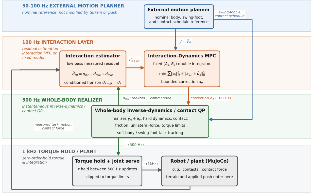
Fixed (A_d, B_d) across gait phase, terrain, and push – environment enters only d_{\text{eff}} , task limits, and realizer.
