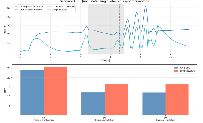
Fig. 4. Scenario F — torso-relative arm error across a quasi-static scheduled single \leftrightarrow double support-mode transition (shaded: right-foot-support model). All controllers stay stable across the contact-model switch; the Kalman gives a modest offset improvement and covariance inflation is neutral (Table VII).
