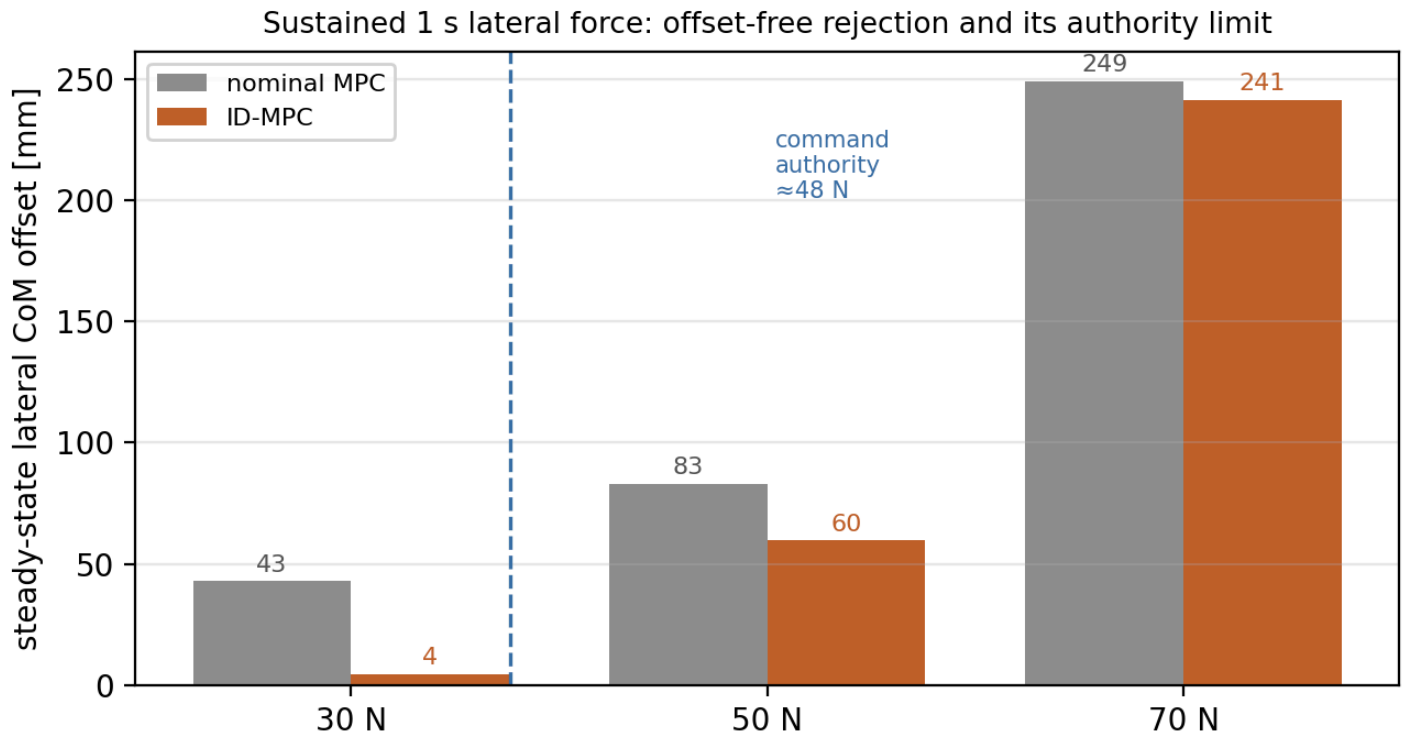
Fig. 8. Steady-state lateral CoM offset under a sustained force; ID-MPC is offset-free within the command authority ( \approx 48 N) and degrades to the nominal droop beyond it.
