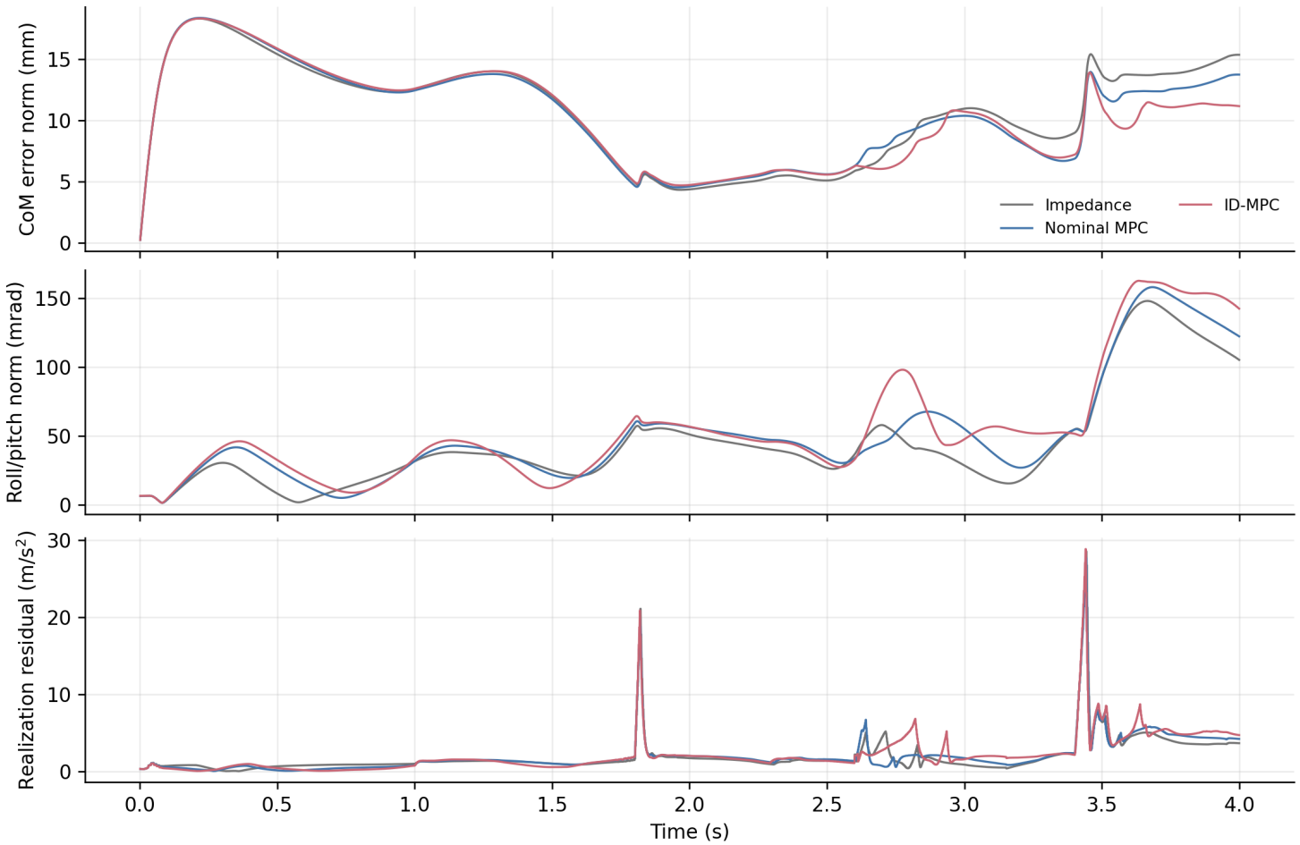
Fig. 5. Representative obstacle response (seed 4200).
