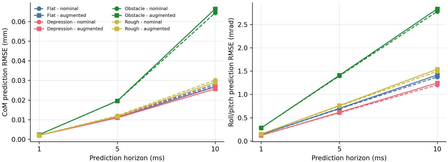
Fig. 3. Interaction-augmented versus nominal prediction.
