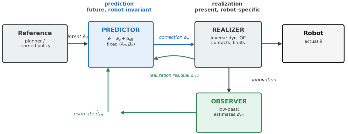
Fig. 2. The interaction-prediction layer sits between the motion planner and the whole-body realizer, estimating d_{\text{eff}} and choosing the task-acceleration correction a_e on the fixed model (4).
