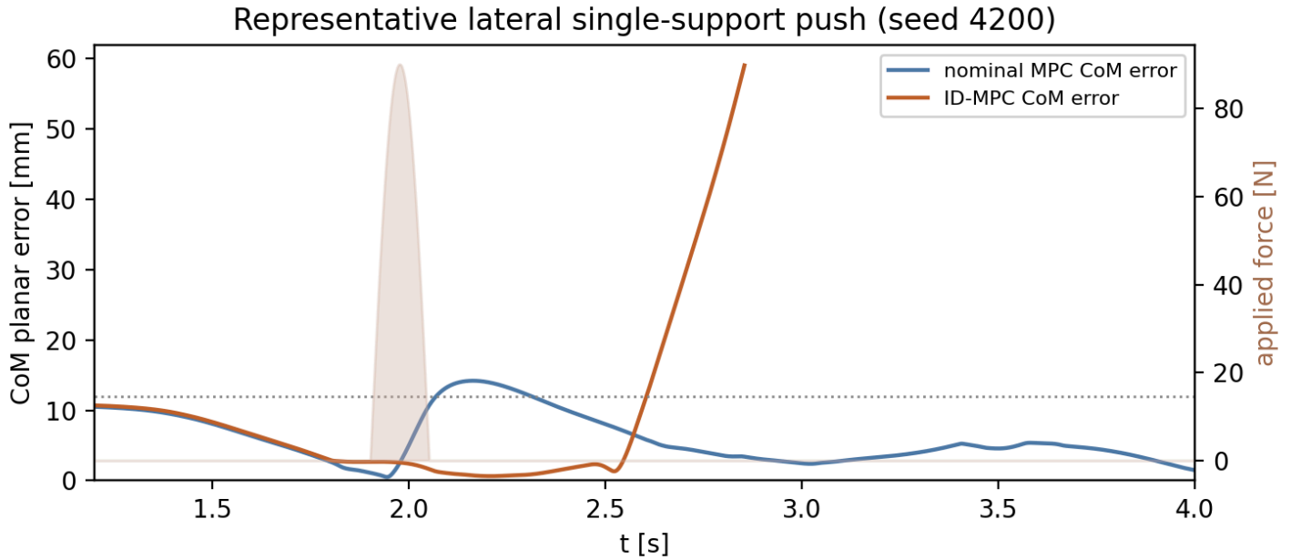
Fig. 7. Representative lateral single-support push: CoM planar error for nominal MPC and ID-MPC, with the applied-force pulse shaded.
