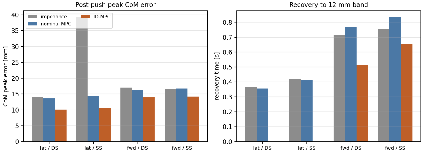
Fig. 6. Post-push peak CoM error and recovery time by controller across the four push conditions.
