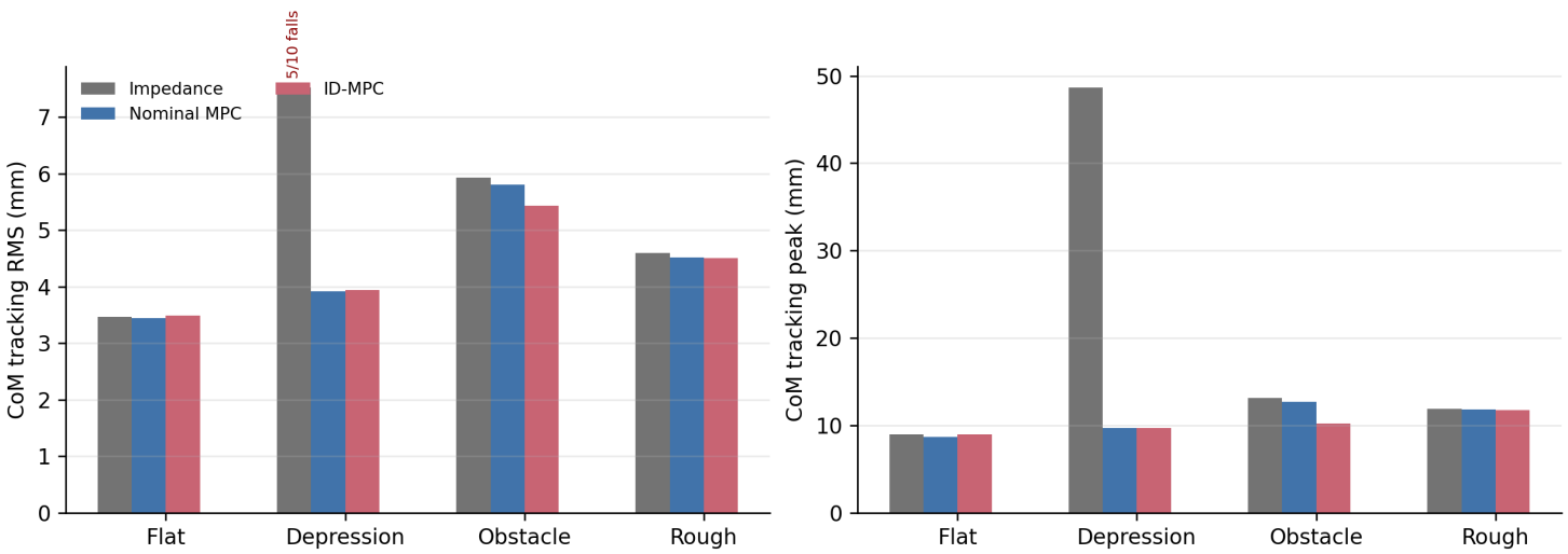
Fig. 4. Uneven-ground tracking summary.
