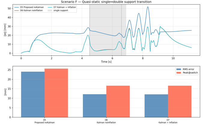
Fig. 4. Scenario F — torso-relative arm error across a quasi-static scheduled single↔double support-mode transition (shaded: right-foot-support model). All controllers stay stable across the contact-model switch; the Kalman gives a modest offset improvement and covariance inflation is neutral (Table VII).
