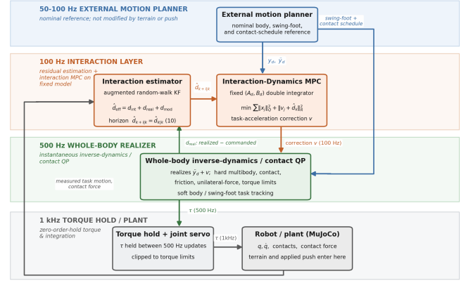
Fig. 1. Interaction prediction with high-rate whole-body realization.
