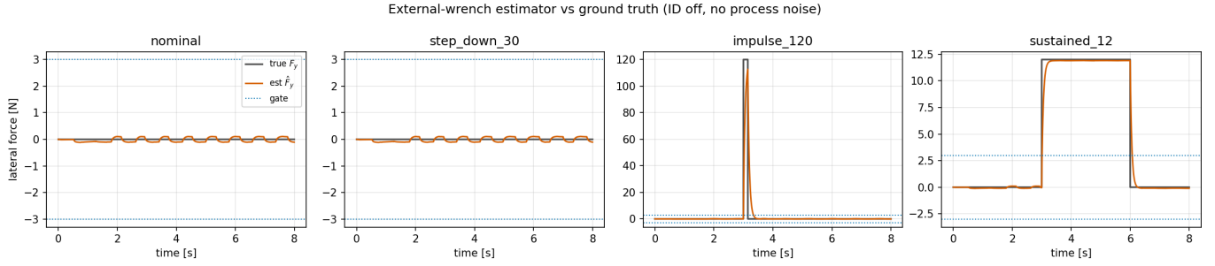
Fig. 3. Estimated horizontal external wrench \hat{F}_{ext} (interaction layer off) versus ground truth across the test scenarios: no false positives on gait and contact transitions, near-instant impulse detection with \sim 0.19 s decay, and \sim 1 N tracking of the sustained force.
