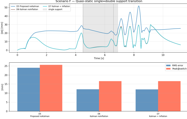
Fig. 4. Scenario F — torso-relative arm error across a quasi-static scheduled single \leftrightarrow double support-mode transition (shaded: right-foot-support model). All controllers stay stable across the contact-model switch; the Kalman gives a modest offset improvement and covariance inflation is neutral (Table VII).
