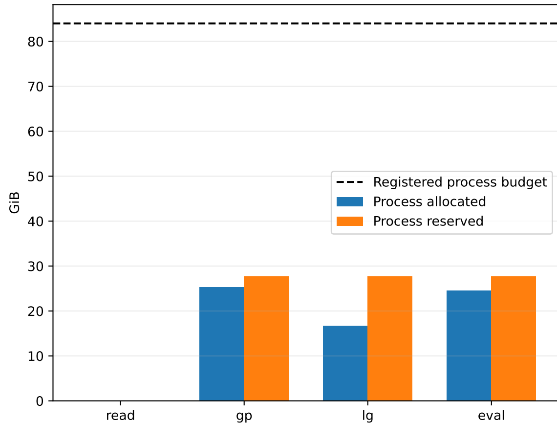
Process CUDA allocator peaks
