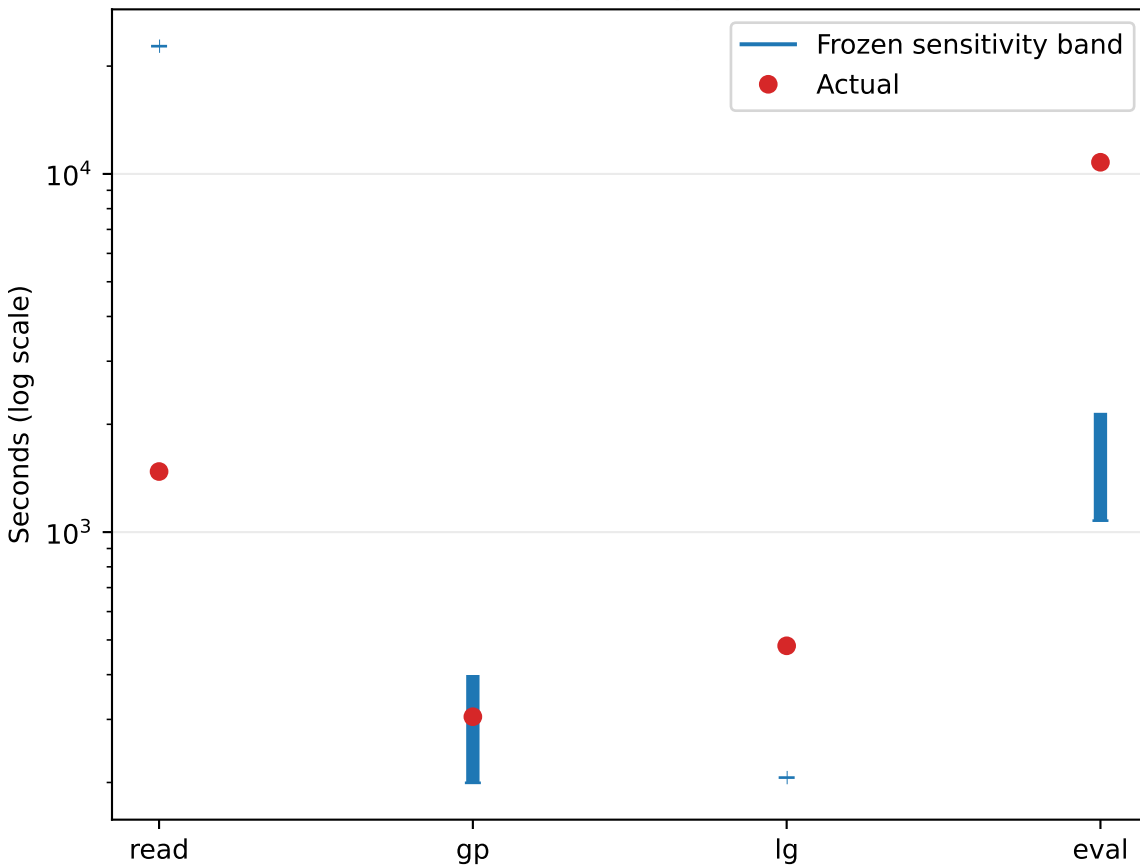
Frozen workload: phase times
