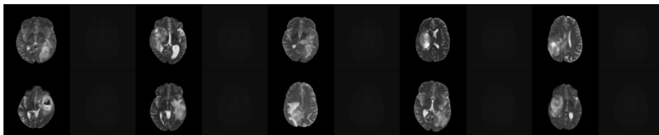
Original/Reconstructed
